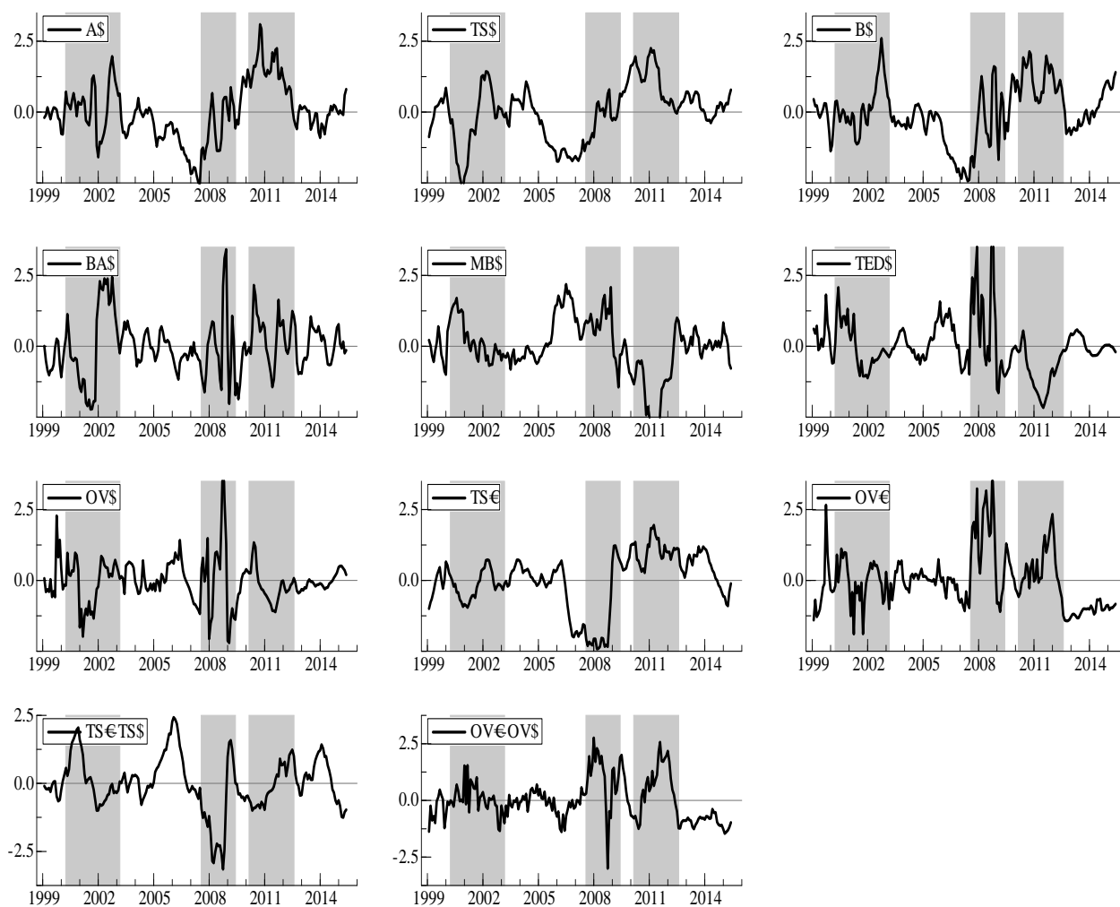
Figure A2: In the figure we plot the estimated interest rate spread anomalies. The plotted series are the US AAA and BAA corporate spreads (A$ and B$); the US BAA-AAA corporate spread (BA$), the US mortgage spread (MB$), the US and EA term spreads (T$$ and TS€), as well as their difference (TS€$); the US Ted spread (TED$); the US and EA overnight spreads (OV$ and OV€), as well as their difference (OV€$). Shaded area refer to financial crises periods for the US and the EA.
