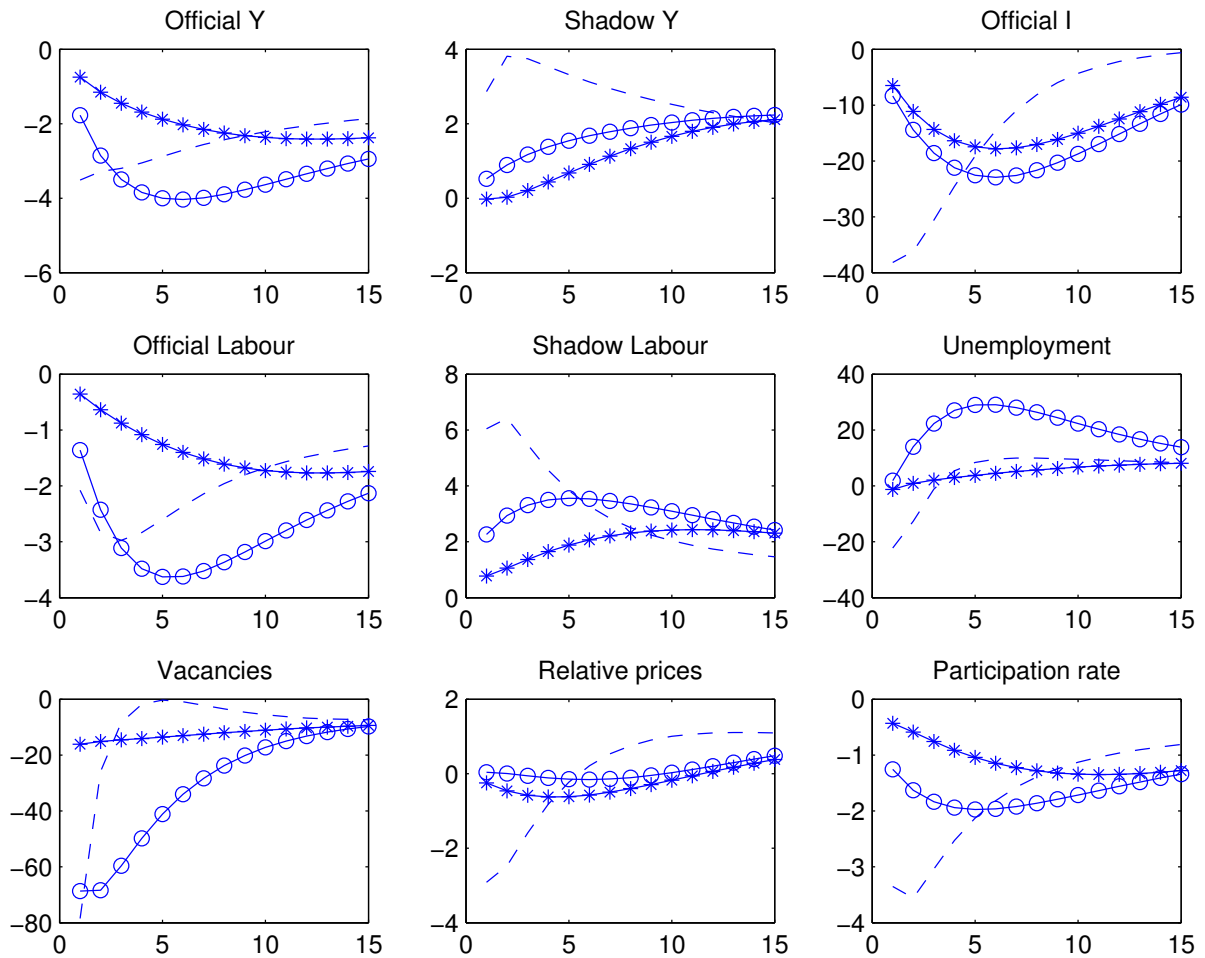
Figure 8: Impulse responses to permanent shock to net worth.
